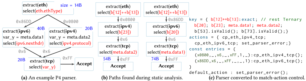
Figure 10: Example illustrating transformation of a parser to a MAT control block by \mu P4C.
